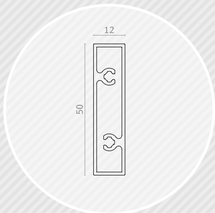
Lame RL50x12
